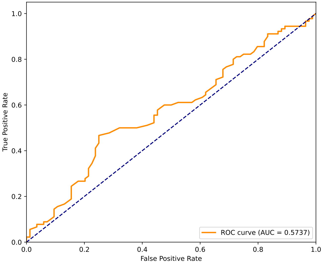
ROC Curve - RandomForest
